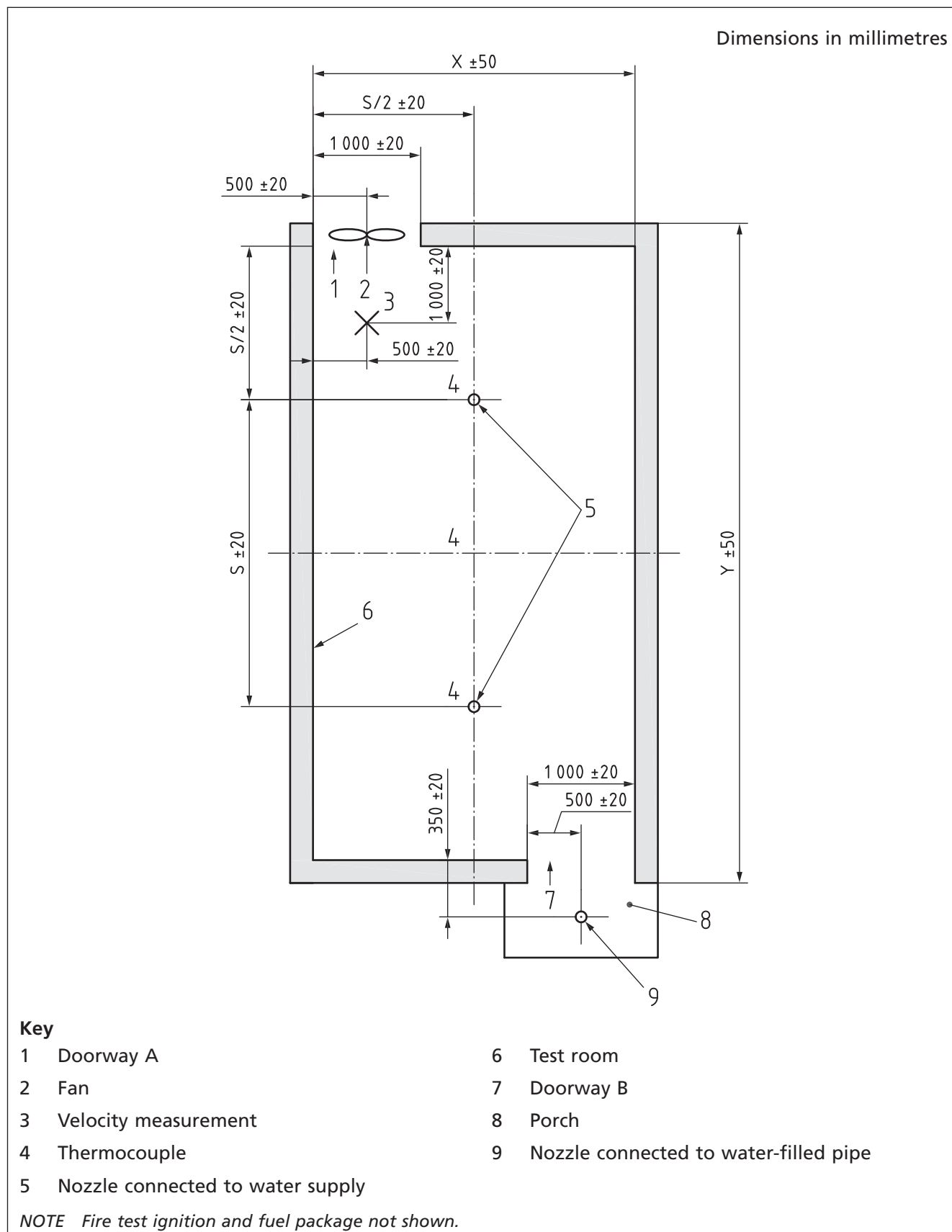
Figure C.6 Ventilation test layout showing a two-nozzle arrangement
